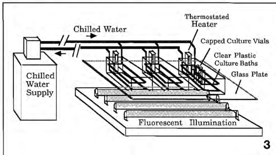
Fig. 3 Illuminated, constant-temperature culture apparatus. A fluorescent fixture provides illumination. Capped culture vials are partially immersed in culture baths. Each bath contains a thermostated, circulating heater to maintain a constant temperature. The chilled water circulating through copper tubing in the water bath is a heat sink. Adapted from Anderson, et al. [4].
